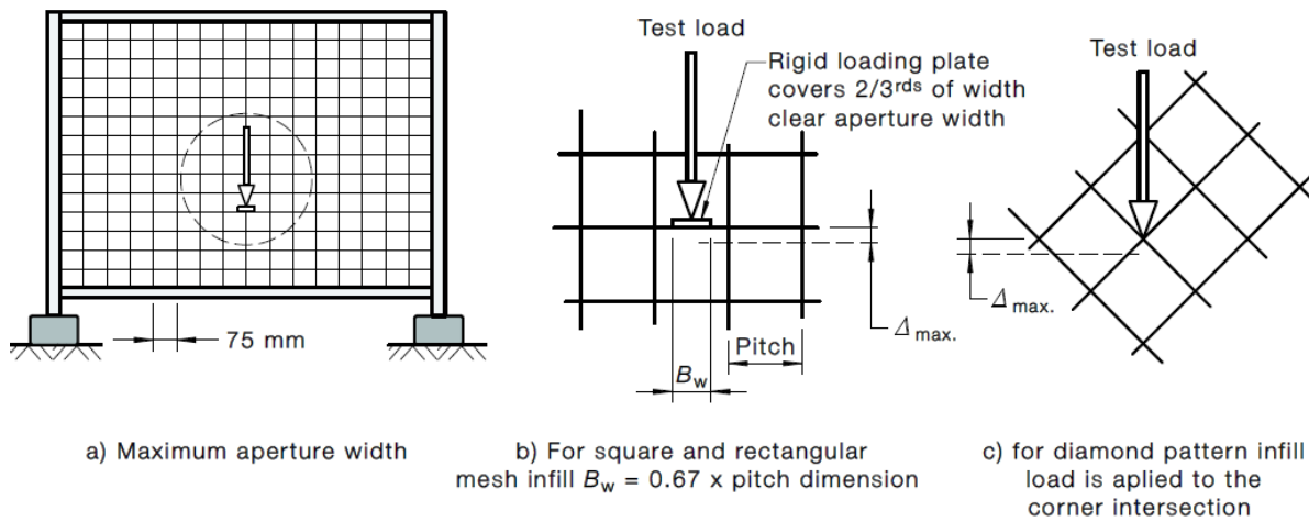
FIGURE 4.4 APERTURE TEST
